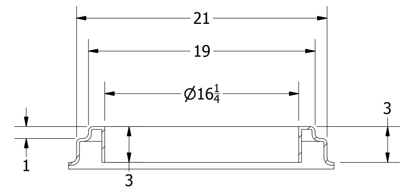
SECTION A-A SCALE 1:8
